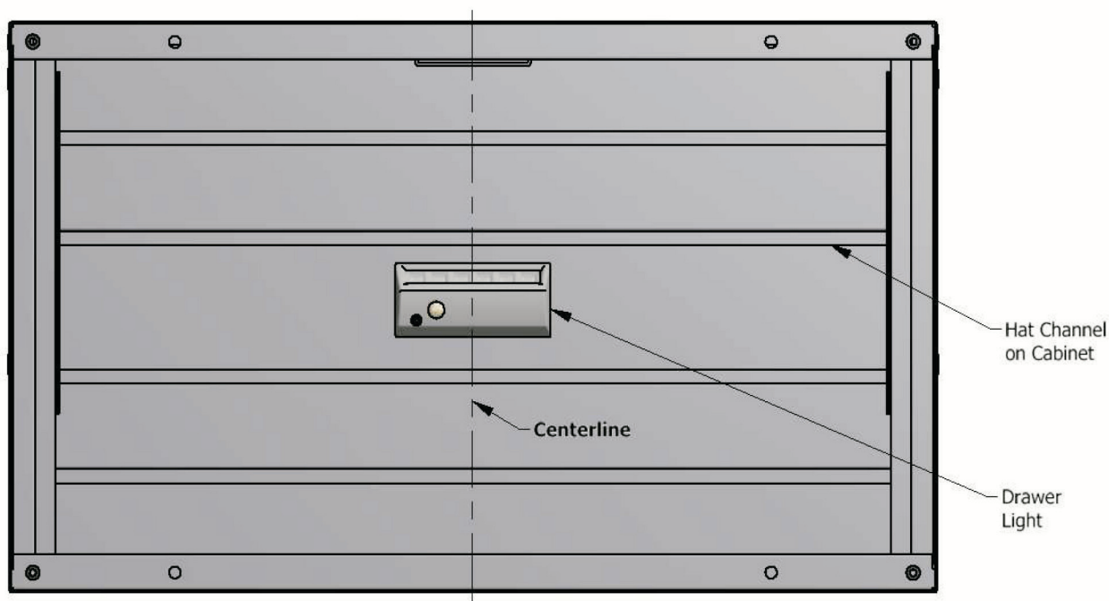
Bottom View of Cabinet (Drawer Removed for clarity)
